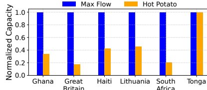
Figure 10: Comparing failover capacity while using max flow and hot potato routing for uniformly distributed terminals capped at 100k population cells.
