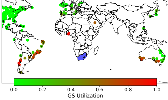
Figure 7: Utilization for different gateways for South Africa when 200k terminals with the GCB policy with no cap.
