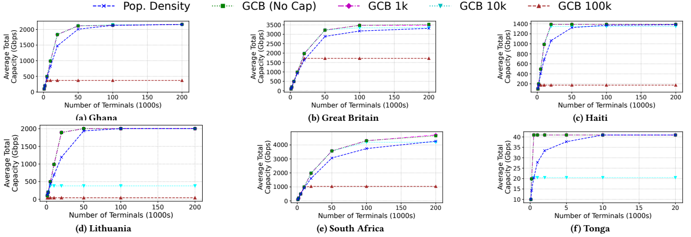
Figure 5: Estimated capacity for various terminal distribution strategies indicates that distributing terminals based solely on population density can reduce network capacity by causing RF contention in densely populated areas and not allocating enough terminals to other areas with RF capacity.
