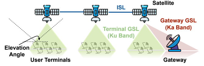
Figure 1: LEO network infrastructure. Radio-based Ground-Satellite Links (GSLs) connect satellites to gateways and terminals. Laser-based Inter-Satellite Links (ISLs) connect satellites to each other.
