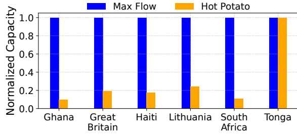
Figure 22: Estimated capacity comparing max flow and hot potato for greedy heuristic based terminal deployment.
