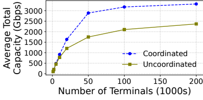
Figure 9: Estimated capacity of Great Britain to distribute terminals by population density, emphasizing the advantages of coordinated spectrum allocation and terminal distribution.
