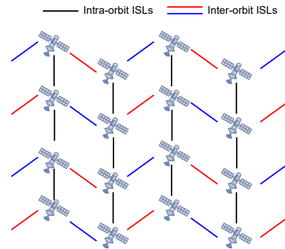
Figure 20: Depicting connectivity in a satellite network with three ISLs. With the +Grid connectivity, both the red and blue inter-orbit ISLs are used while for three ISLs, only the blue ones are used.
