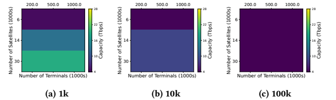
Figure 13: Impact of capped terminal distribution on South Africa's estimated capacity with an expanding LEO network, highlighting how usable capacity quickly plateaus due to RF bottlenecks in densely populated areas.
