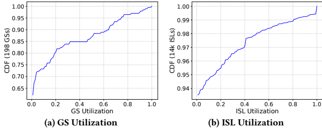
Figure 6: CDF of GSL and ISL utilization for South Africa when 200k terminals with the GCB policy with no cap.
