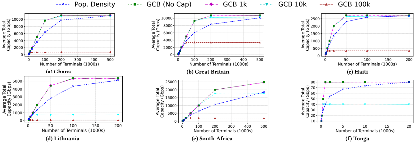
Figure 16: Even with a different wireless model with increasing the Ku band data rate to 2.5 Gbps (config C in Table 2) and increasing the number of satellites to 14k, the estimated capacity for various terminal distribution strategies follows similar trends.
