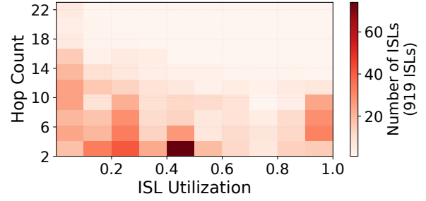
Figure 8: Utilization and number of hops from the terminals for ISLs for the South Africa case when 200k terminals are distributed using the GCB policy with no caps.
