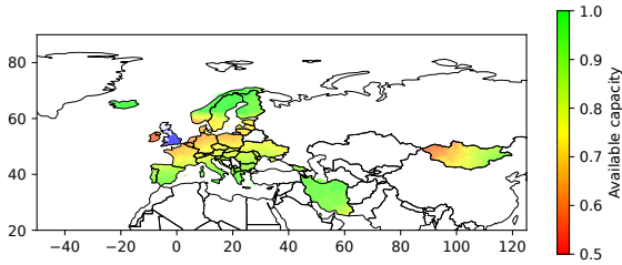
Figure 14: Great Britain’s failover traffic significantly affects deprioritized incumbent traffic across most of Europe and Asia. Neighboring countries lose up to 50% of their LEO network capacity, highlighting the potential need for international coordination in cases of infrastructure failure.
