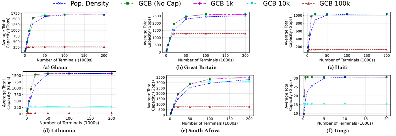
Figure 15: Even with a different wireless model with reducing the Ku band data rate to 0.956 Gbps (config B in Table 2), the estimated capacity for various terminal distribution strategies follows similar trends.
