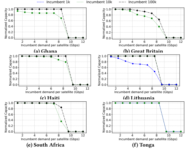
Figure 24: Estimated capacity for different incumbent demands per satellite.
