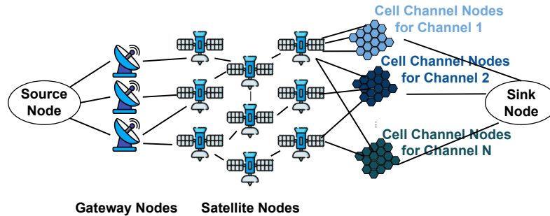
Fig. 9. Construction of CosmoSim graph. Cell channel nodes represent the same set of cells, where each cell is covered by a different set of channels.
